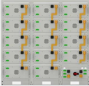
Battery String-5224
